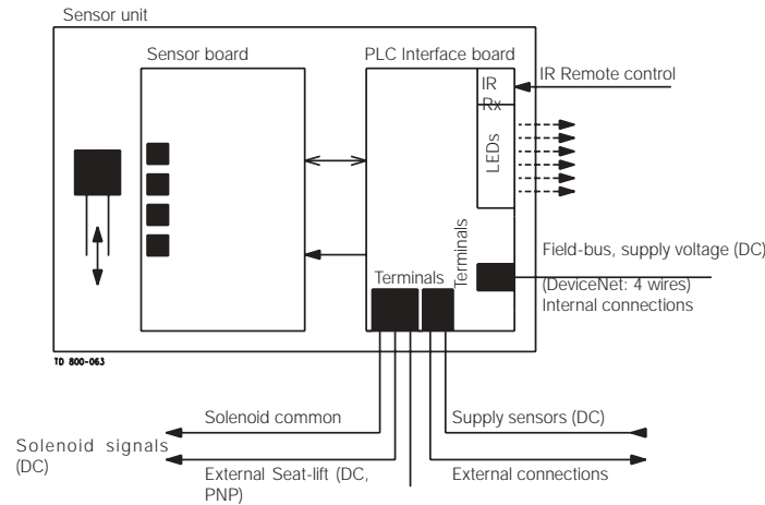
Type: Alfa Laval “No Touch” Sensor System
