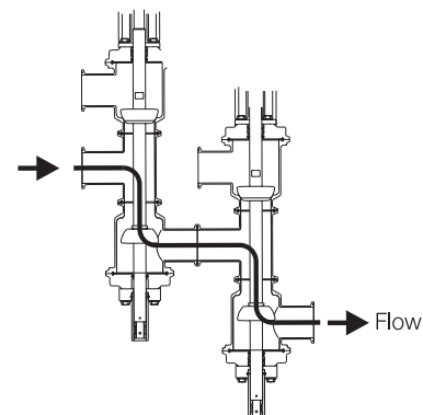
Reverse-Acting Flow
