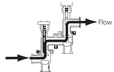
Standard Valve Flow
